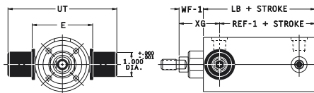
HEAD TRUNNION MOUNT (NFPA MT1)
