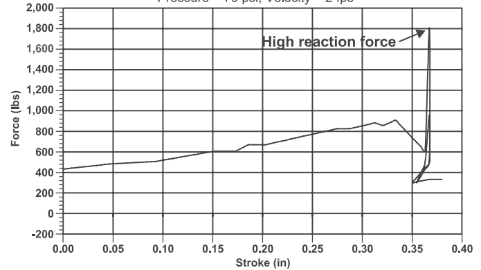
Pneumatic Cushion - Stroke vs Force
