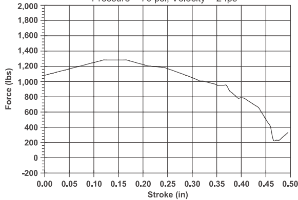
NuCushion - Stroke vs Force
