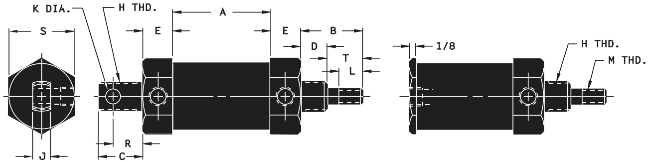
Models FTM/FTMR Swivel Mount Cylinders
