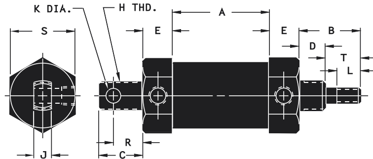
Models MTM/MTMR Swivel Mount Cylinders
